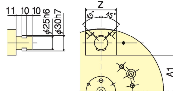
08", 10", 12" jaw mounting part dimensions (Jaw's shaft)
