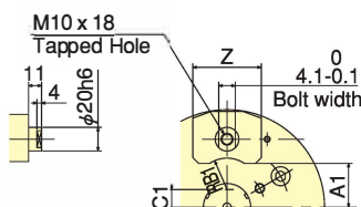
05", 06" jaw mounting part dimensions (Jaw's shaft)
