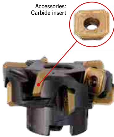
Accessories: ZFR 250 arbor milling cutter
